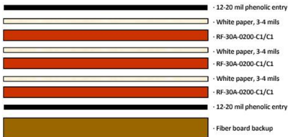
Figure 5 – Typical TLF-35A rout stack-up
