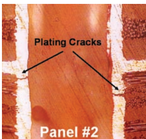
Figure 13. Sample of Barrel Crack Failure, Standard FR4.
